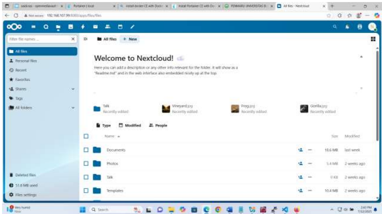
Gambar 9. Tampilan Nextcloud
