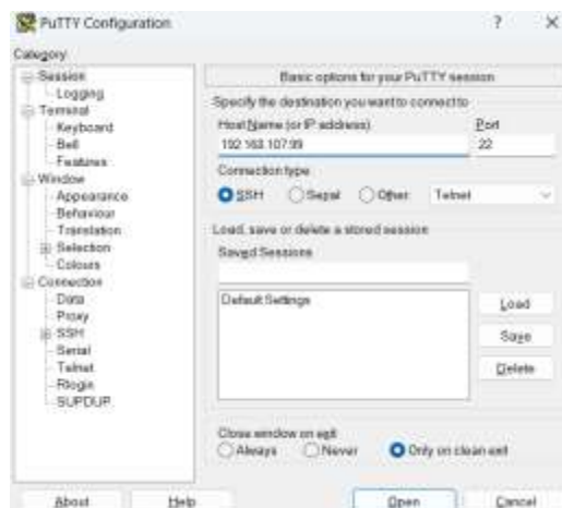
Gambar 3. Remote Server
