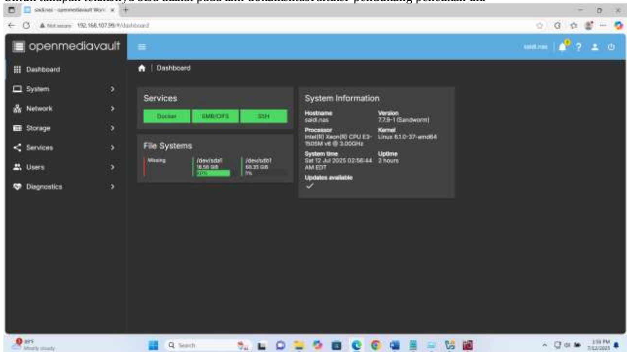
Gambar 2. Tampilan openmediavault
