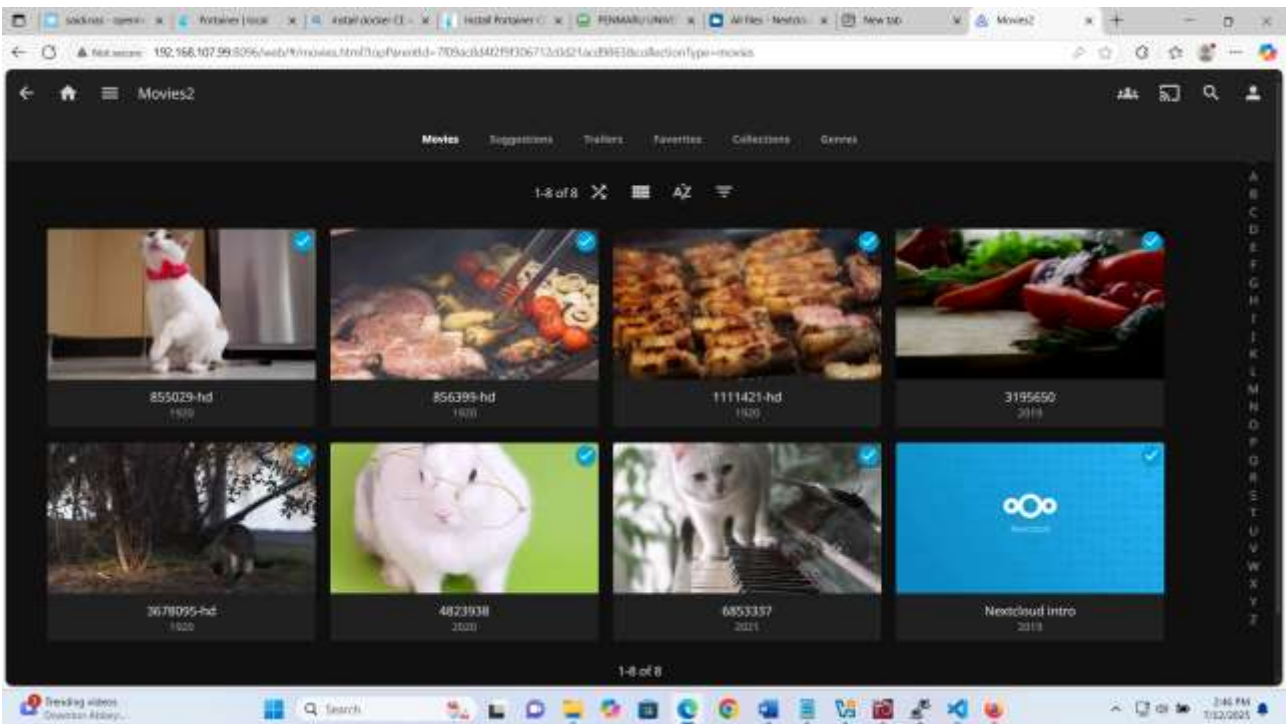
Gambar 10. Tampilan Jellyfin
