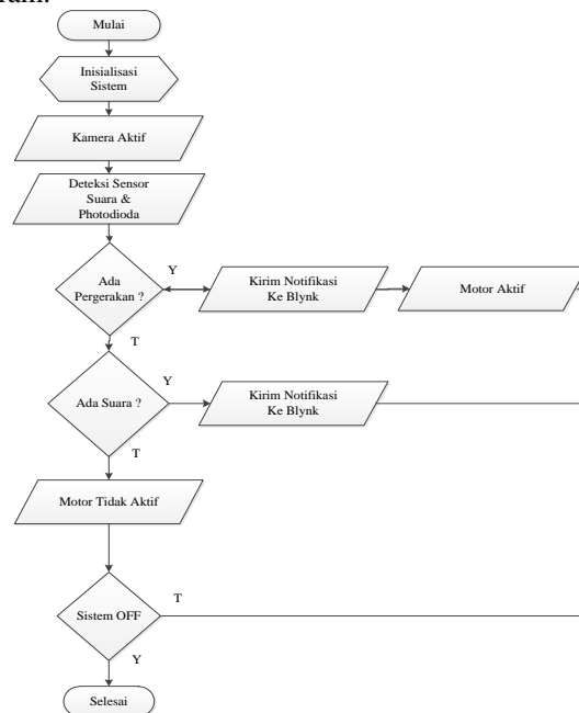
Gambar 7. Flowchart Sistem
