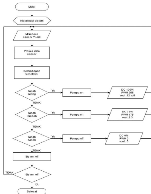
gambar 2.3 Flowchart sistem
