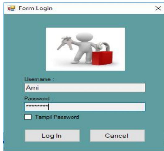
Gambar 4.1 Form Login
