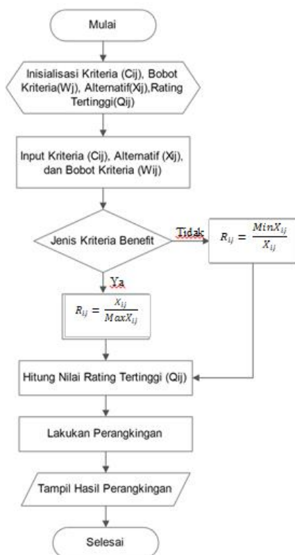
Gambar 1. Flowchart Metode WASPAS
